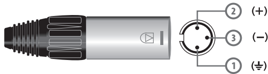
INPUT Balance input XLR-F
