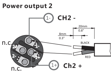
Power output-speaker output NL4 Speakon Connection method
