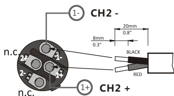
SPEAKON Power output-speaker output NL4 Speakon Connection method
