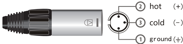
INPUT Balance input XLR-F
