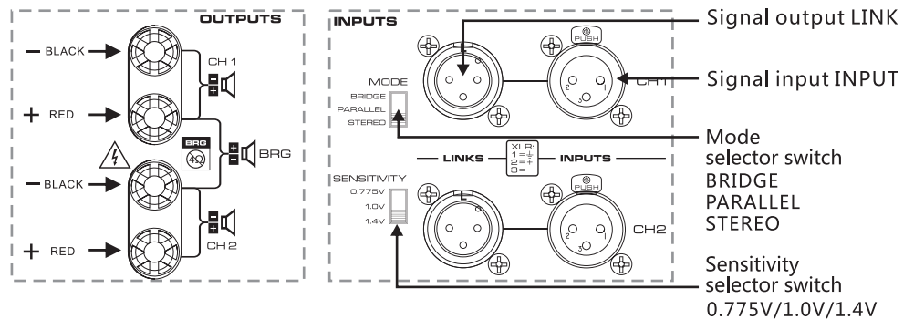
Signal connector
