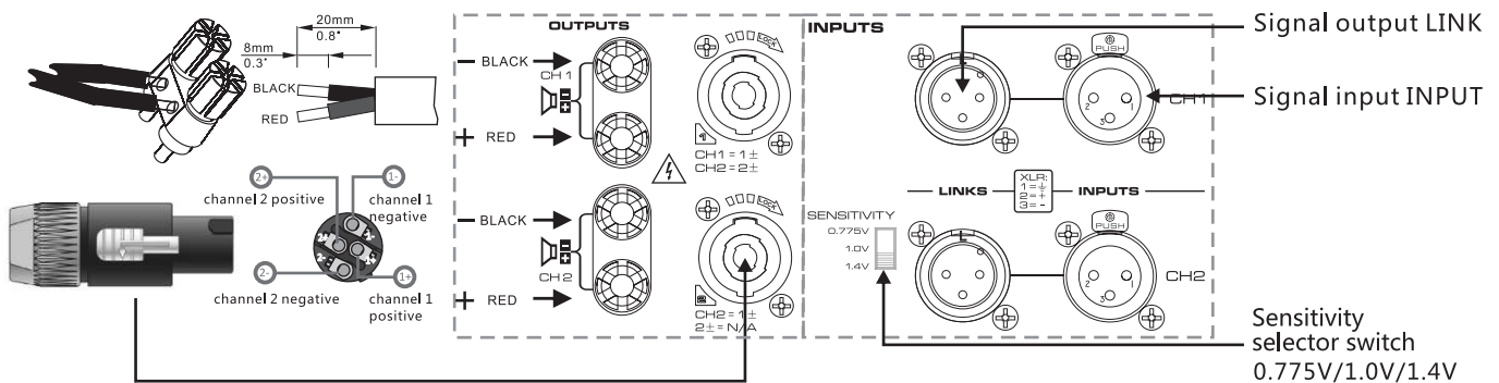
Signal connector
