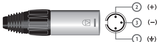
INPUT Balance input XLR-F
