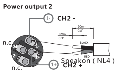
SPEAKON Power output-speaker output NL4 Speakon Connection method
