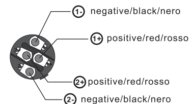
Speaker speaker (NL4) (Only for EX5200)
