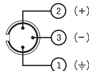
INPUT Balanced male XLR
