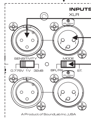
INPUT Balanced male XLR
