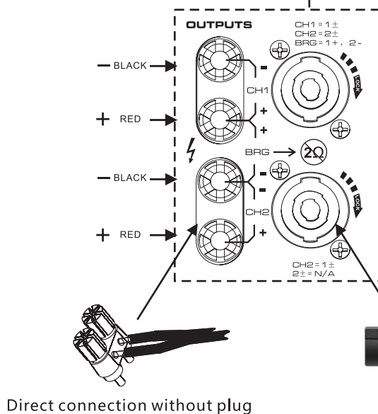
Speakon ( NL4 )
