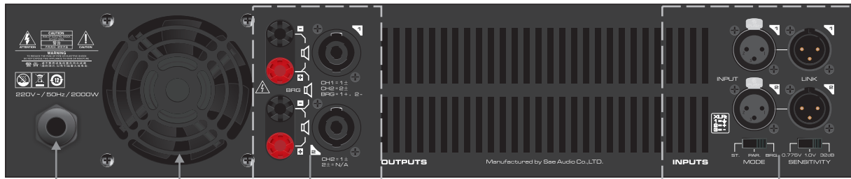
Power cable
