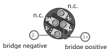
OUTPUT 1 BRIDGE
