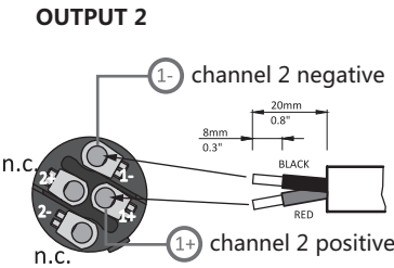
Speaker power output - speaker output NL4 SPEAKON connection mode
