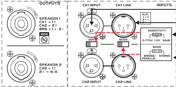
Signal connector
