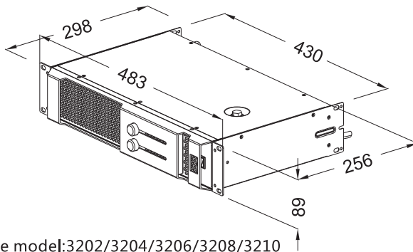
Suitable model:3202/3204/3206/3208/3210
