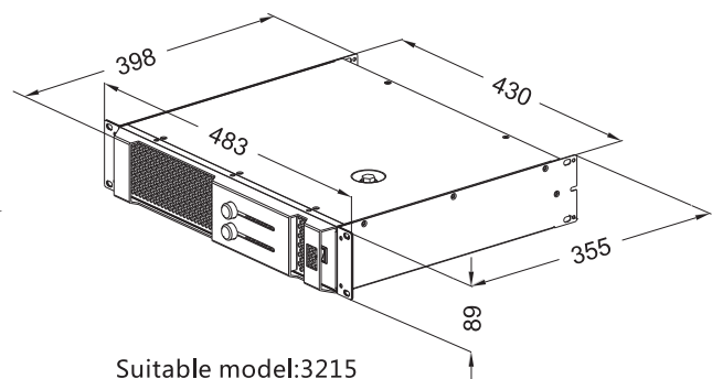
Suitable model:3215
