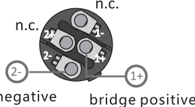
OUTPUT 1 BRIDGE
