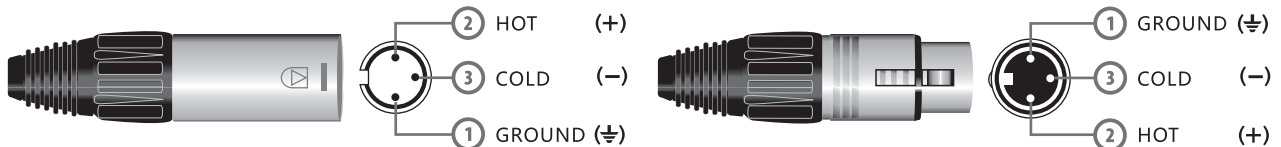
INPUT Balanced connection male XLR
