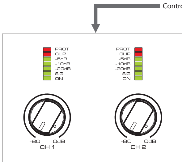
CH1-CH2 → Gain Controller Knob 300° volume knob from 0 to -80dB.
